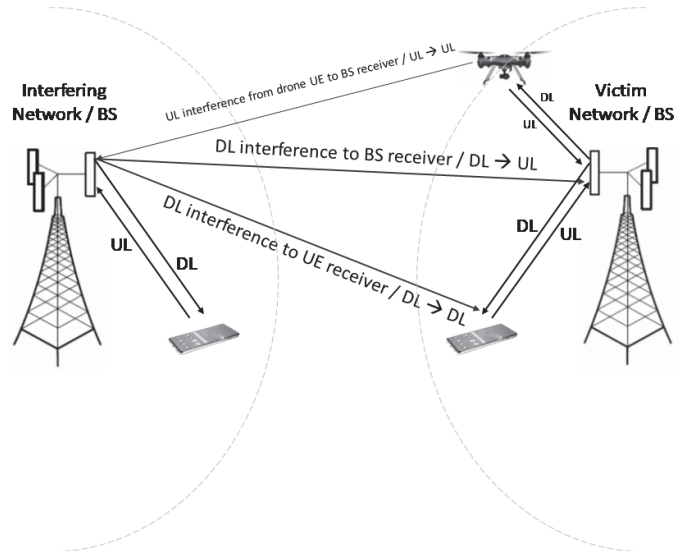
Fig. 1. Interference modes
