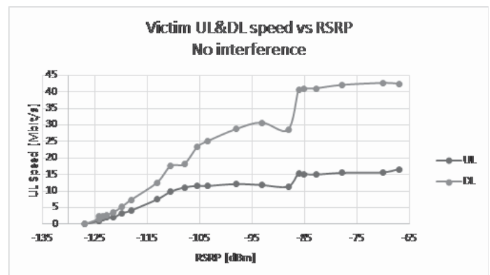
Fig. 5. Victim side UL & DL speeds as a function of RSRP
