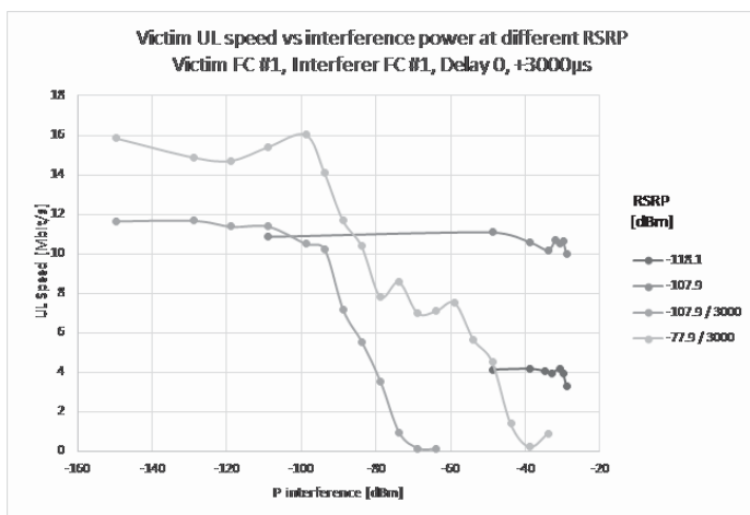
Fig. 11. Victim UL speed, frame configuration #1 and #1, delay 0 / 3000 \mu s
