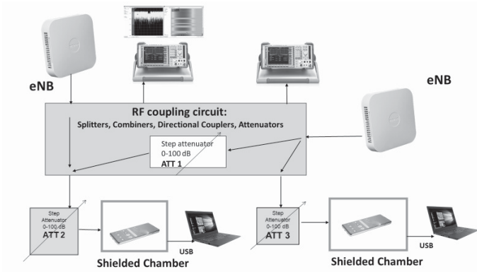
Fig. 3. Laboratory measurement test bench
