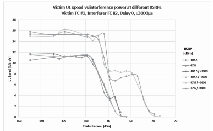
Fig. 13. Victim UL speed, frame configuration #2 and #1, delay 0 / \pm 3000 \mu s
