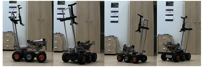
Fig. 4. The movement of a mobile robot around its axis
