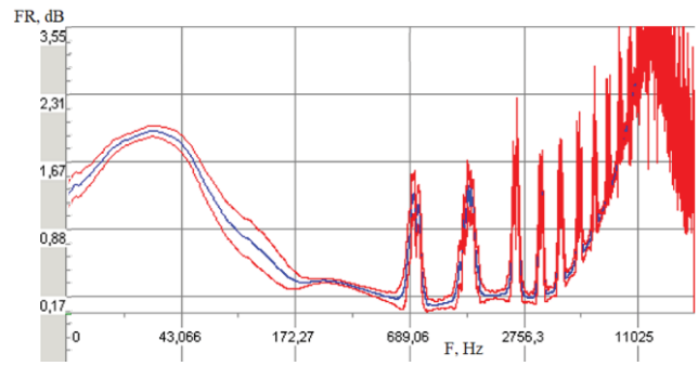
Fig. 10. FR of the equalizer is formed by changes in the instantaneous spectra of the real signal (blue -average value FR, red - dispersion of values FR)
