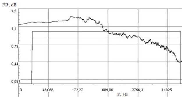
Fig. 8. FR of the audio processor T.C. Electronics DBMax in hardware backup studio
