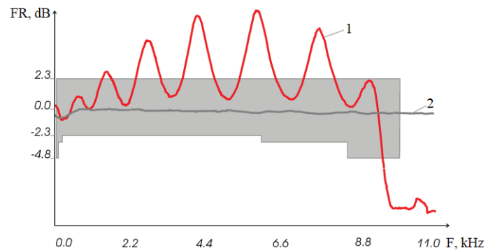
Fig.6. FR of the Optimod audio processor, Orban, formed from a real signal (1) and ARGO (2)
