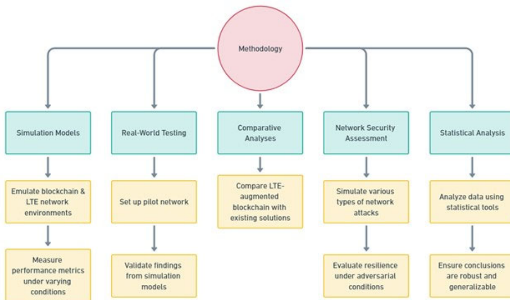
Fig. 1. Methodology Flowchart
